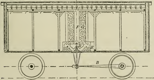
Refrigerating apparatus for transport cars according to Trapp.
